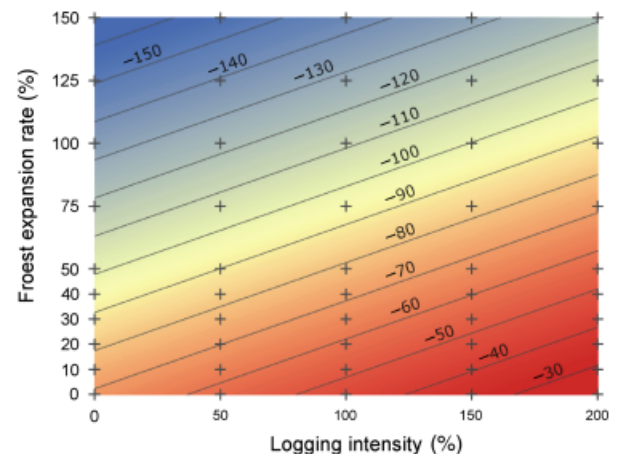
Fig. 6 Total carbon sink strength [ \text{Tg C} ] between 2008 and 2100 for different scenarios of logging intensity ( 100\% = 5000 \text{ ha yr}^{-1} ) and forest expansion ( 100\% = \text{all currently unused farmland} \sim 728\,000 \text{ ha} ). Crosshairs mark modeled scenarios; isolines denote identical sink strength across different scenarios.
