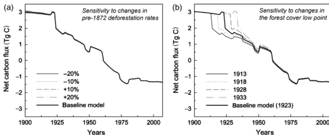
Fig. 7 Changes in the net carbon flux between 1900 and 2007 compared with the baseline model when varying pre-1872 deforestation rates by \pm 10\% and \pm 20\% (a) and when shifting the low point in forest cover by \pm 5 and \pm 10 years (b).
