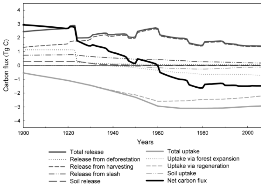
Fig. 4 Carbon fluxes due to land-use change in western Ukraine between 1900 and 2007. The net carbon flux is the total release of carbon (positive flux for emissions) minus the total uptake of carbon. Total release consists of carbon emissions following forest clearing or logging via biomass that is removed from a site (release from deforestation or from harvesting), via decaying biomass on site (release from slash), or from the soil carbon pool (soil release). Total uptake consists of carbon that is stored in regrowing vegetation on abandoned sites (uptake via forest expansion) or after harvesting (uptake via regeneration) and in the soil (soil uptake).
