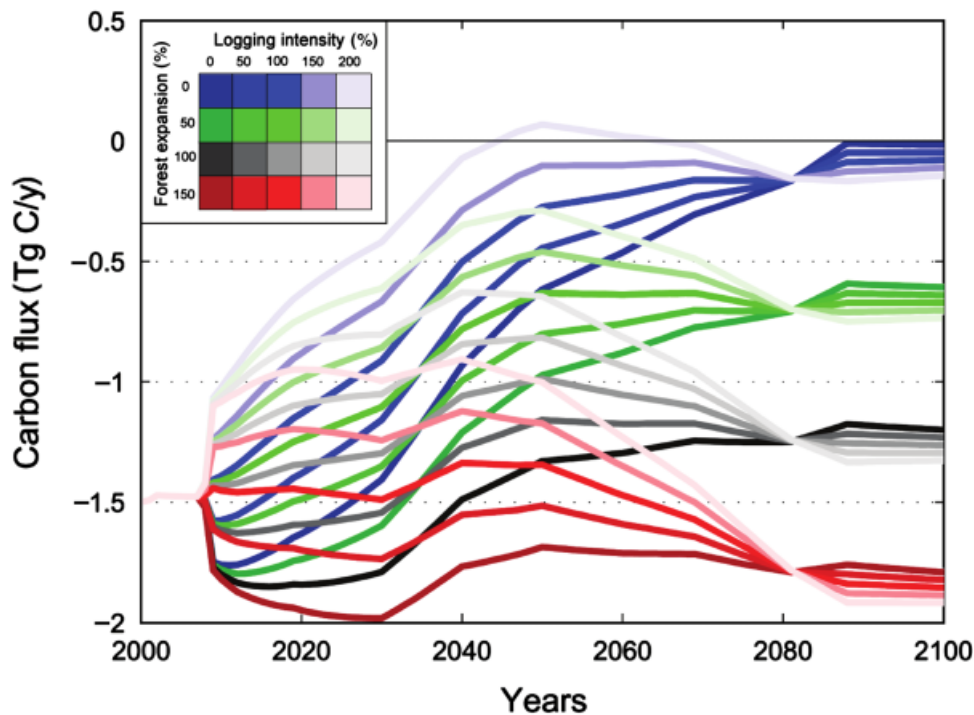
Fig. 5 Net carbon fluxes for different scenarios of logging intensity and forest expansion on currently unused farmland. Higher logging intensities lead to a higher initial release and higher sequestration in the second half of the simulation period (due to regrowing vegetation). Higher forest expansion rates result in more carbon being stored in vegetation and thus more negative net carbon fluxes.
