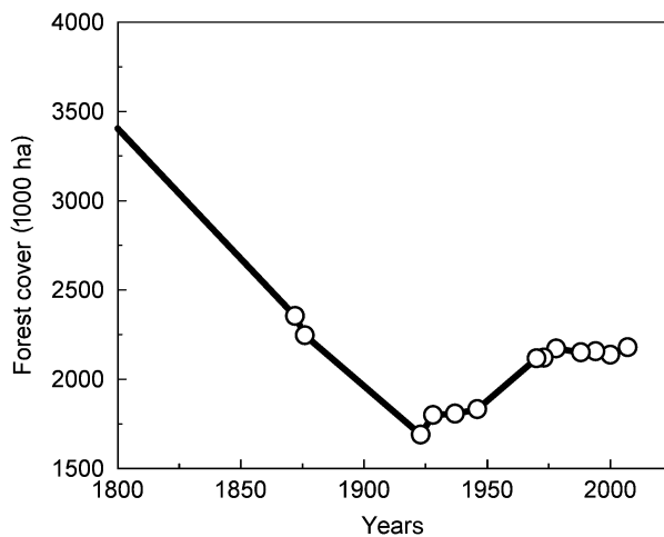
Fig. 2 Forest cover changes in western Ukraine between 1800 and 2007. Estimates are from historic land-use surveys (1872, 1876, 1923, 1928, 1937), statistical yearbooks (years 1946, 1970, 1973, 1978), and remote sensing images (1988, 1994, 2000, 2007). Presettlement forest cover for the study region was estimated at 75% (see 'Materials and methods' for details).
