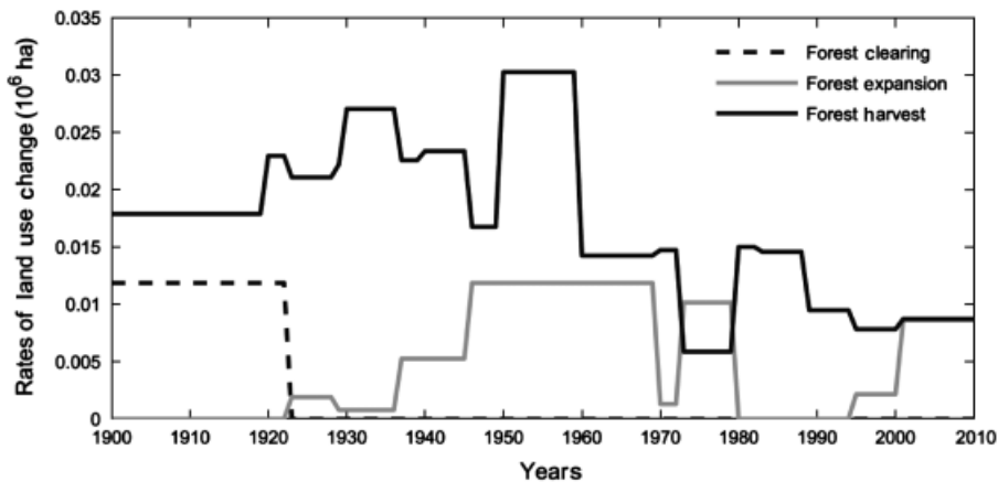
Fig. 3 Rates of permanent forest clearing, forest harvesting, and forest expansion for the time period 1900–2007 used as input data for the carbon bookkeeping model.
